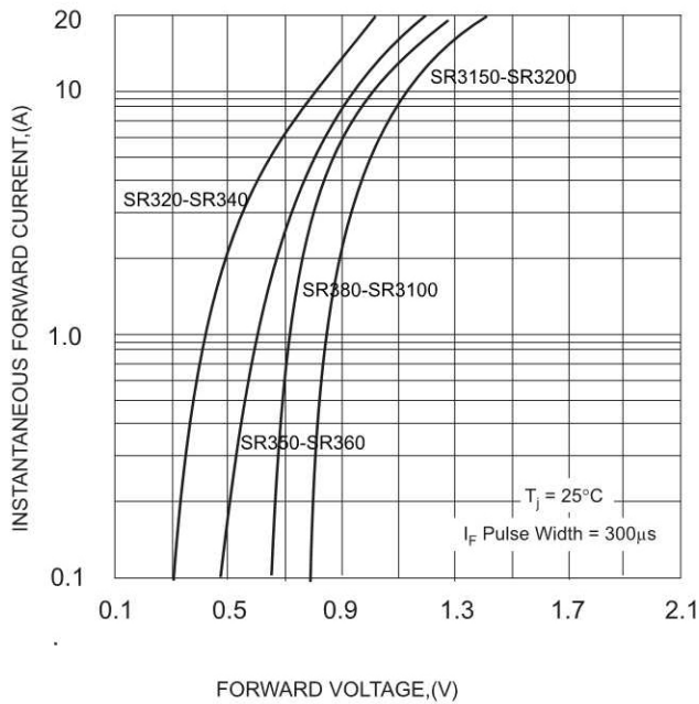
FIG.1-TYPICAL FORWARD CHARACTERISTICS
