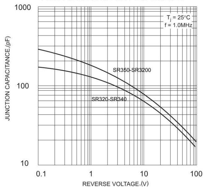
FIG.5-TYPICAL JUNCTION CAPACITANCE
